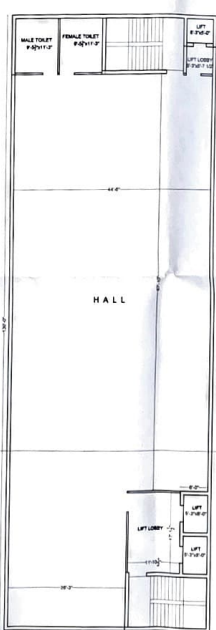
SIXTH FLOOR PLAN TOTAL COVD AREA = 5488.84 SQFT
